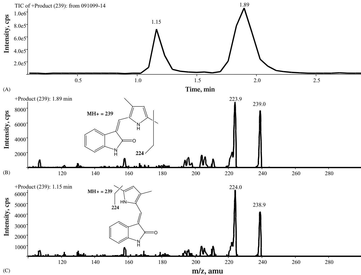
Fig. 2. A typical chromatogram (A) of the Z- and E-isomers, and their spectra (B and C). Fifty microliters of 250 ng/ml standard solution (in 50% acetonitrile) exposed to a light for 30 min was injected onto the LC/MS/MS system and the daughter ion of 239 scan was monitored.
